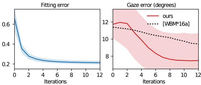
Figure 11: Fitting error and gaze error for the Columbia dataset [SYFN13]. Line is median, filled region is interquartile range. Our second-order optimization strategy converges much faster than previous first-order methods [WBM*16a].
