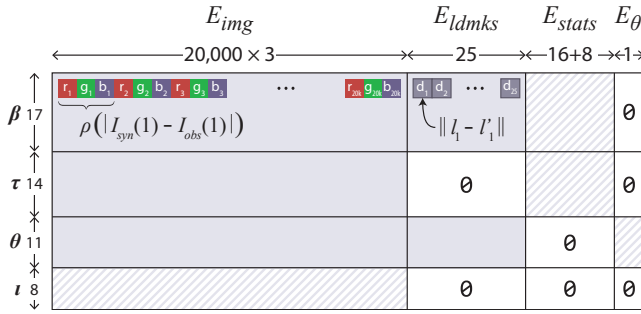
Figure 8: The non-zero structure of our Jacobian J_r for a 200 \times 100px eye region. J_r is calculated entirely on the GPU. Dashed regions represent sparse blocks.
