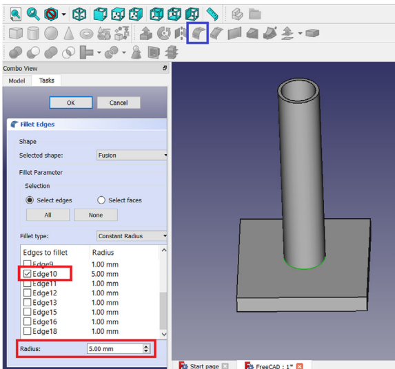
Figure 5: Filleting the edge connecting the rectangular base and the cylindrical tube in FreeCAD. The relevant edge is selected in the interactive view. Then, the 'Fillet' option in the toolbar is chosen. The boxes on the menu on the left show the corresponding edge reference and the fillet parameter.
