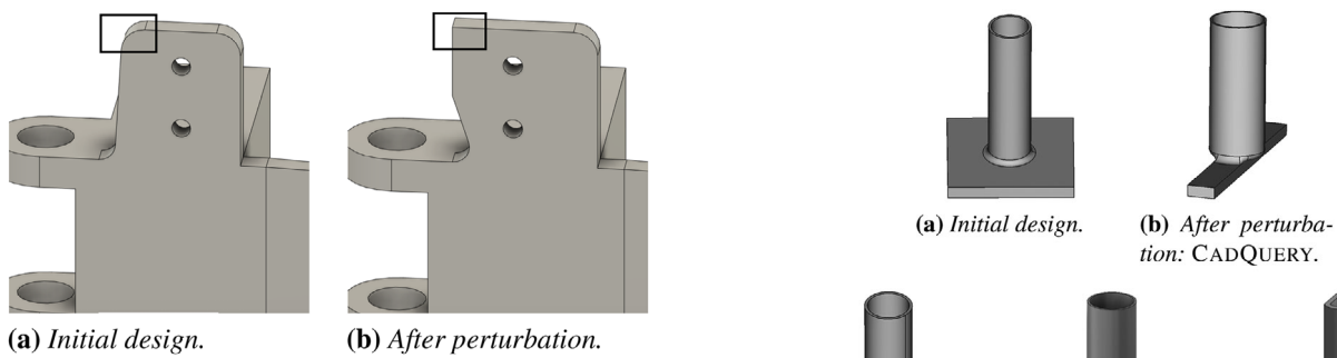
Figure 2: The side bracket design fails to fillet the intended edges (see black box) after the length of the top edges is increased.
