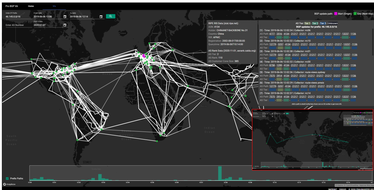
Figure 4: Real world use case: Large European route leak from AS21217 sends traffic through China Telecom. Immediately, the large quantity of BGP updates (white paths) shows the global impact of this event. The color code on the right side shows how the routing hierarchy was interrupted. The AS path shows that the Tier 3 AS21217 is in between two Tier 2 ASes, which in general should not be the case. In the bottom right, one path is highlighted by the user. It shows clearly how the path made a detour over China before being routed to the US.
