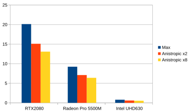
Figure 6: Performance in Giga-texel per second on different GPUs.
