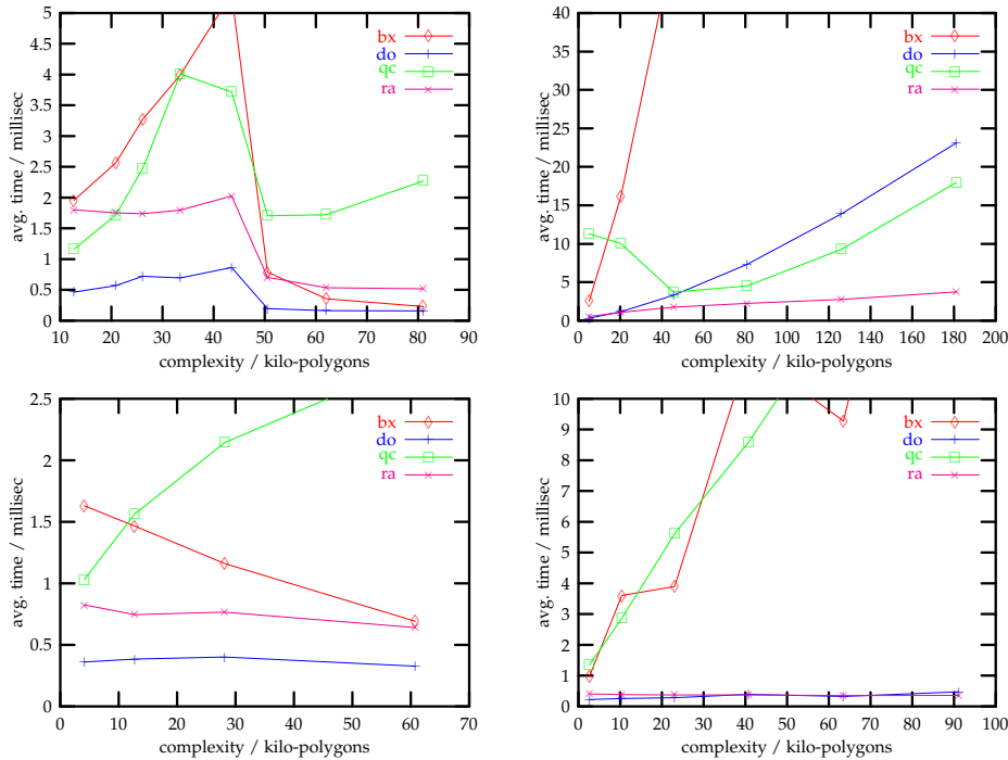
Figure 3.44: Comparison of the 4 hierarchical collision detection algorithms. The objects from top left: door lock, hyperboloid, car body, torus.
