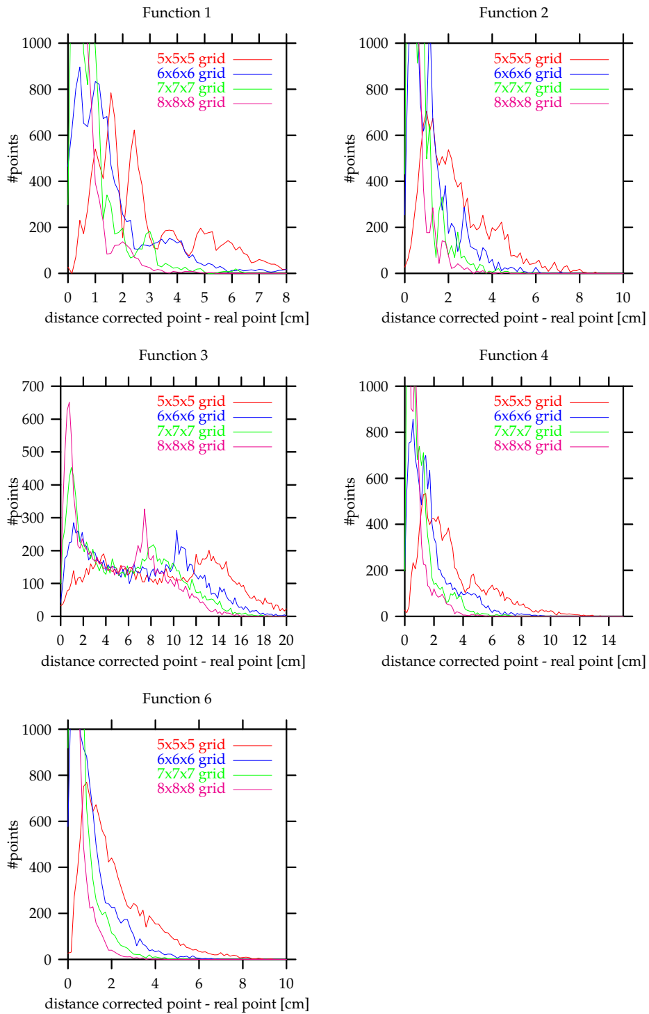
Figure 4.25: Histograms of the translational error after HMQ interpolation with optimal R^2 for different grid resolutions ( 5 \times 5 \times 5 \dots 8 \times 8 \times 8 ).
