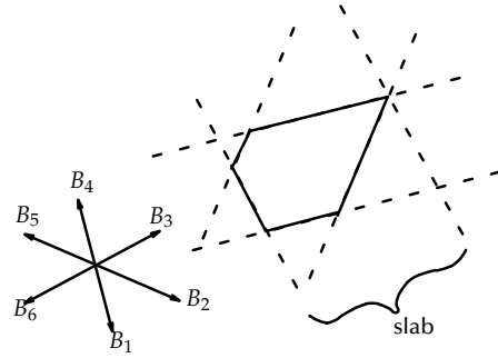
Figure 3.32: k -DOPs can be viewed as intersection of k/2 slabs.
