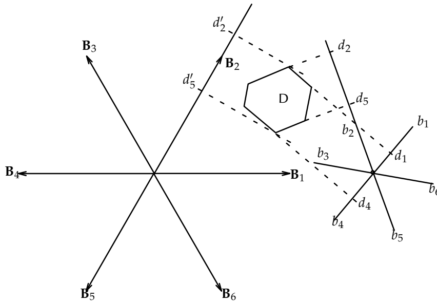
Figure 3.34: A rotated DOP can be enclosed by an aligned one by computing new plane offsets d'_i . Each d'_i can be computed by an affine combination of 3 d_{j_i} , 1 \leq i \leq 3 (2 in 2-space). The correspondence j_i depends only on the affine transformation of the associated object and the fixed orientations \mathbf{B}_i .
