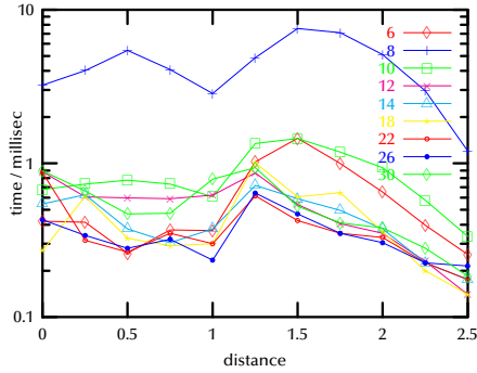
Figure 3.38: Collision detection time for two tori, each with 10,000 polygons. The distance is, as always, measured between their centers. Each graph corresponds to a particular k .
