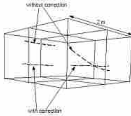
Figure 4.21: The dashed lines show the locus of points as reported by the tracker when the sensor is moved along a perfectly straight line. The dash-dotted lines show the same lines with correction. The error of the corrected positions from the true positions is less than 4 cm.
