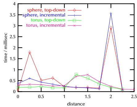
Figure 3.51: The collision query time depends on the distance of the two objects (approx. 23,000 pgons/object). I believe that the incremental algorithm does not perform better due to a significantly higher number of secondary level cache misses.
