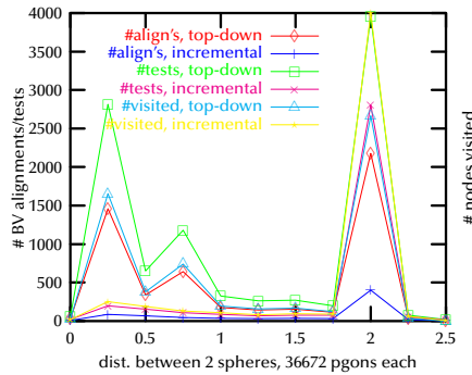
Figure 3.46: The number of BV test, DOP alignments, and nodes visited depends on the distance between the objects.
