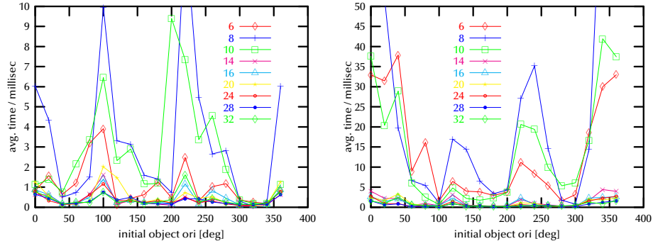
Figure 3.36: The effect of an object’s coordinate frame on collision detection performance can be significant. Left: two car bodies (60,000 polygons each), right: door locks (43,000 polygons each). The plots have been generated by the benchmark procedure outlined in Section 3.5.10. The time shown is the collision detection time averaged over “interesting” distances. The locks are different in that most of the polygons are in the interior, because it has many parts on the inside. This might explain the “inversion” of the shape of the curve.
