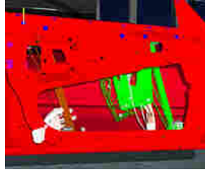
Figure 5.9: The window regulator has to be installed with two hands; the “ghost” paradigm signals collisions.
