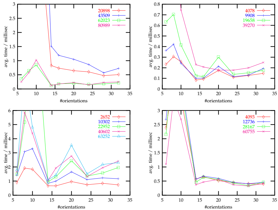
Figure 3.40: Average collision detection time for various objects of the “suite” depending on different k (from top left: door lock, hose, sphere, car body). The average was calculated over the “interesting” distance range and over all object coordinate frames. Each object has a “radius” of 1.
