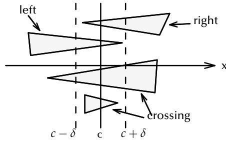
Figure 3.26: For splitting a set of polygons by a plane, geometrical robustness can be achieved by giving the plane a certain “thickness”.
