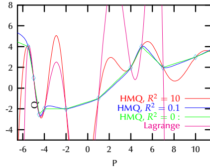
Figure 4.19: 1D examples of HMQ interpolation functions through 10 points with various R^2 parameters. For R^2 = 0 the function is piecewise linear. The Lagrange interpolant exposes fatal oscillations.
