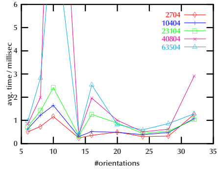
Figure 3.39: The same data as in the figure to the left (each graph corresponds to a certain distance). This graph provides some evidence that the optimal k does not depend on the distance between objects. For all other objects in the “suite”, similar graphs were obtained.
