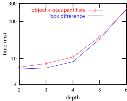
Figure 3.60: Performance gain by incremental maintaining of octrees of dynamic scenes. A depth of 0 corresponds to one cell only. Both variants use occupant lists, but one of them visits only cells which are in the box difference.
