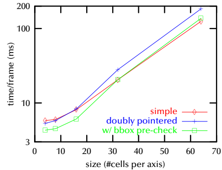
Figure 3.61: Comparison of the simple and the doubly-pointered grid data structure. Grid updating plus generation of “close” object pairs with 100 objects. The third curve is with the additional pre-check whether the new and the old bounding boxes (in integer coordinates) are the same.
