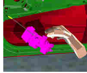
Figure 5.10: The object-on-the-lead paradigm allows to verify assembly. The object is not linked rigidly to the hand.
