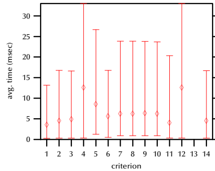
Figure 3.29: Average performance of the splitting criteria. Criterion 1 creates the best BoxTrees.
