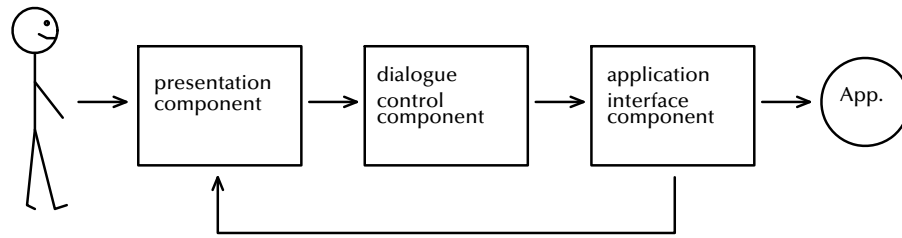
Figure 2.2: The Seeheim model modularizes UIMSs into three components.
