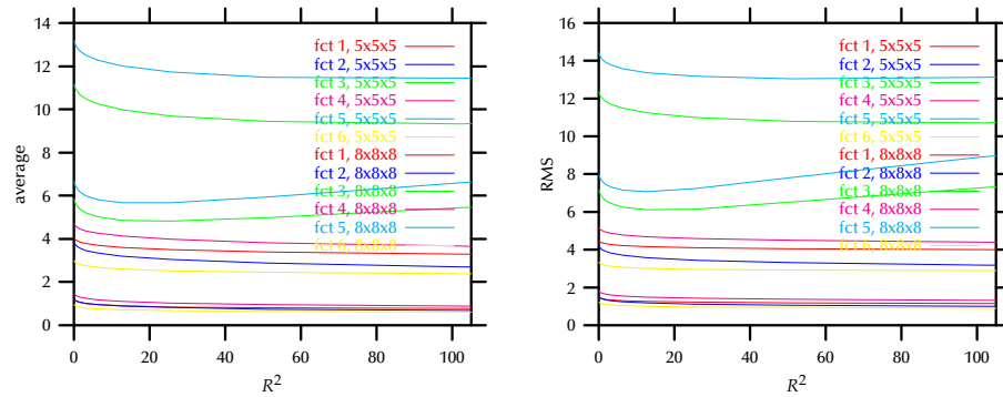
Figure 4.26: The dependence of the remaining distortion error on the parameter R^2 (left: average error; right: RMS).
