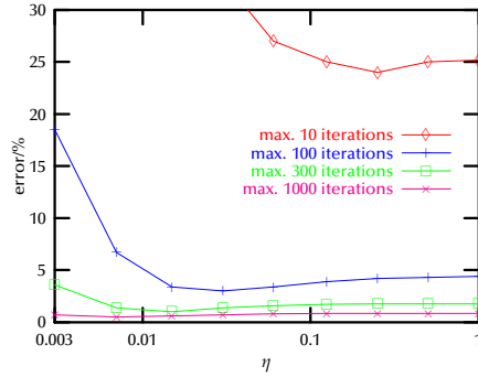
Figure 3.8: Impact of \eta and the max. number of iterations on the correctness of the separating planes algorithm. The error is the number of times where the separating planes algorithm returned with “collision”, but there was none, in fact.
