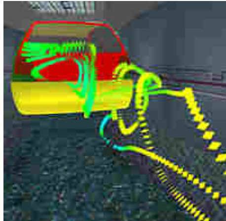
Figure 5.17: Immersive CFD investigation: color-coded particles indicate the flow and pressure around a VW Polo. Data courtesy of Volkswagen AG.
