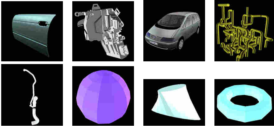
Figure 3.42: A suite of test objects. They are (left to right): the sheet metal of a car door ( \approx 3,000 polygons), the lock of a car door ( \approx 20,000\text{--}80,000 polygons), body and seats of a car ( \approx 4,000\text{--}60,000 polygons), a section of pipes ( \approx 120,000 polygons), a hose ( \approx 4,000\text{--}40,000 polygons), sphere ( \approx 3,000\text{--}90,000 polygons), hyperboloid ( \approx 5,000\text{--}180,000 polygons), torus ( \approx 3,000\text{--}90,000 polygons). (Data courtesy of VW and BMW)
