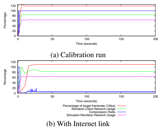
Figure 3: Simulation of Pollution Demonstrator.
