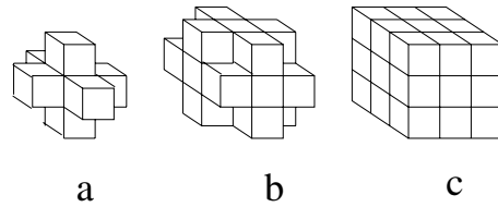
Figure 2: The sets of 3D voxels that are N -adjacent to the voxel at the center. a) N = 6 . b) N = 18 . c) N = 26 .
