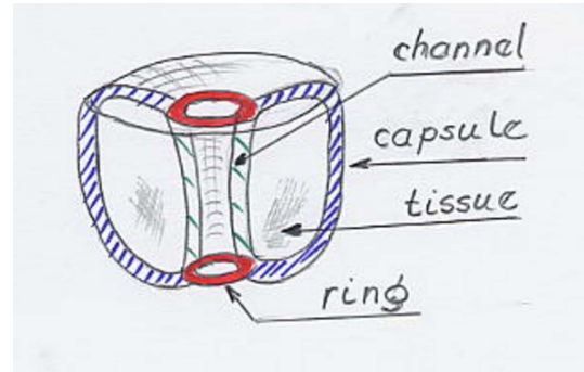
Figure 11: Sets of voxels.
