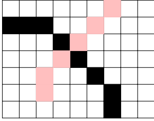
Figure 3: An 8-connected curve penetrating through another 8-connected curve.
