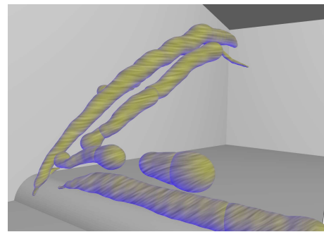
(a) Blunt fin; vortex hulls.
