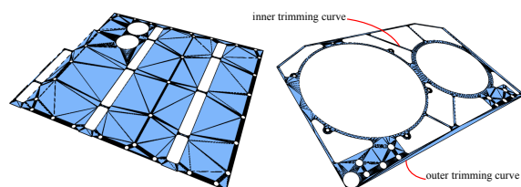
Figure 1: Trimmed surface tessellation produces a lot of ill-configured triangles.
