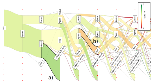
Figure 8: This figure shows a meta-data filter including only NPS response callers where the colour is also associated with the NPS score (Q1, Q5, Q6). You can see that customers who ended the call in the shortest time frame (i.e. IVR → Queue → Agent → End) are satisfied with the service (Transition a). Callers who were placed on hold for the second time are dissatisfied (Transition b).
