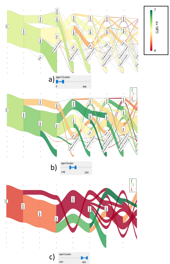
Figure 7: This image shows the meta-data brush applied to the agent duration axis where colour is mapped to the NPS (Q6). You can see that image b) is generally more green than the other two, and image c) is more red. The journeys don't vary too much between a) and b), but c) looks different due to the longer nature of the calls, and less of them.
