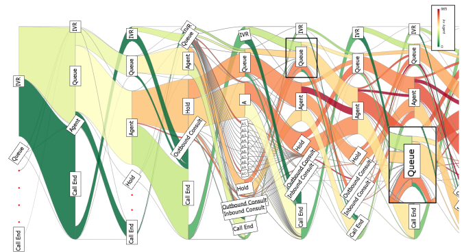
Figure 3: This figure demonstrates a typical RiverState view as state transitions flow between time-oriented events (Q2). The agent state at timestep 5 has been broken down into 11 agent sub-states corresponding to different departments in the call centre (Q4). The bottom state at each axis represents a call end (Hang up state). Edges transitioning from these states represent repeat callers (Hang up → IVR).
