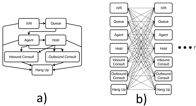
Figure 2: This figure shows the differences between a) typical FST diagrams and our method of displaying the data b) whereby each state node is repeated for each time step.
