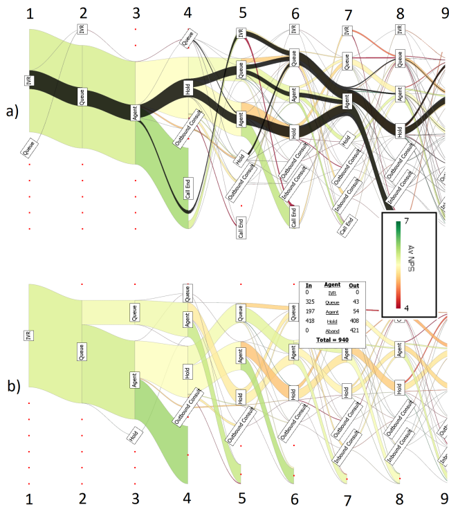
Figure 4: This figure demonstrates the interactive features of the RiverState application. Image a) shows a filter applied to the agent state at axis 3. This also demonstrates the traceroute feature where the user has moved their mouse over the agent state at timestep 7. Image b) shows a meta-data filter applied so that only callers who responded to an NPS survey about the call are shown (Q1,Q2). Both images are coloured by this NPS score. Image b) also demonstrates the details on demand mouseover feature which displays the numerical data behind the transitions at the selected state.
