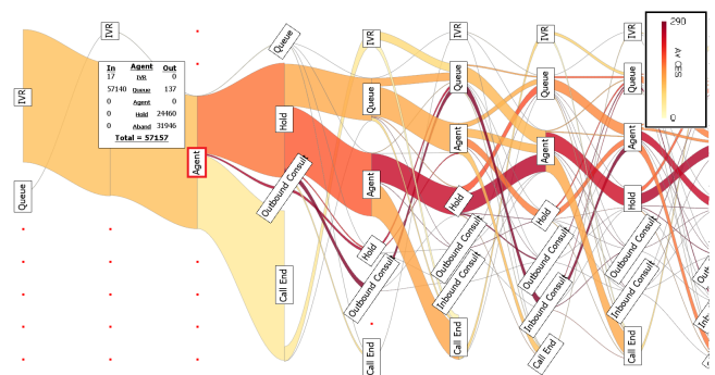
Figure 5: This image shows the beginning of an average call (Q2). IVR → Queue → Agent. At that point slightly more than half of calls terminate there, and the other half continue to be placed on hold. The detail on demand tooltip is used to show the exact number of calls entering and exiting the states.
