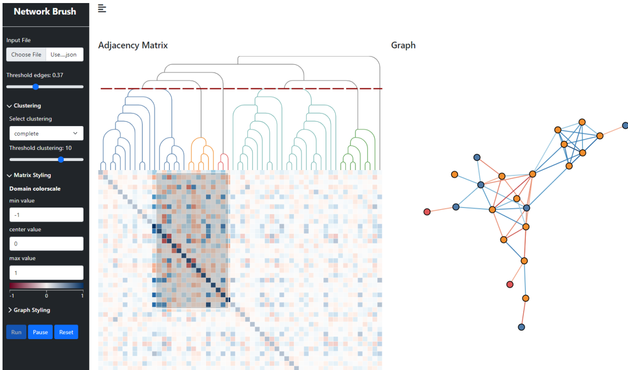
Figure 1: Full overview of MOBS' functionality; in detail exploration of subgraphs from a larger biological correlation network after hierarchical clustering is applied. Relations between proteome (blue), clinome (yellow-orange) and metabolome (red) nodes, that are considered important (absolute value > 0.37 ), are shown.
